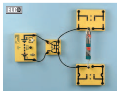
Experiment 065: Force caused by a flexible current-carrying conductor within the inhomogeneous magnetic field of a bar magnet
